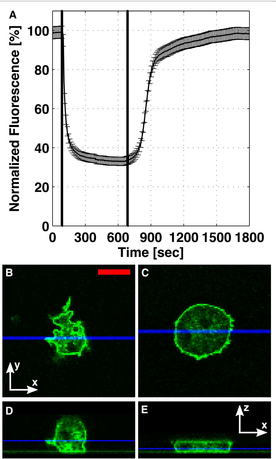
Figure 7 Characterization of the single layer microfluidic device. (A) The channel was filled with 100 \mu\text{M} fluorescein, and the intensity in the middle of the device was recorded. Between t = 85 s (line 1) and t = 685 s (line 2), the syringe pump withdrew 250 \mu\text{l/h} of the fluorescein through the device, leading to a drop in the channel height. This flow rate was used to flatten cAR1-GFP cells. Confocal x-y scans are shown for a cAR1-GFP cell (B) before and (C) during flattening. (D, E) show the corresponding x-z sections. The blue lines in (B, C) show the y-values for the sections (D, E), and the blue lines in (D, E) show the z-value of images (B, C). Scale bar: 10 \mu\text{m} .
